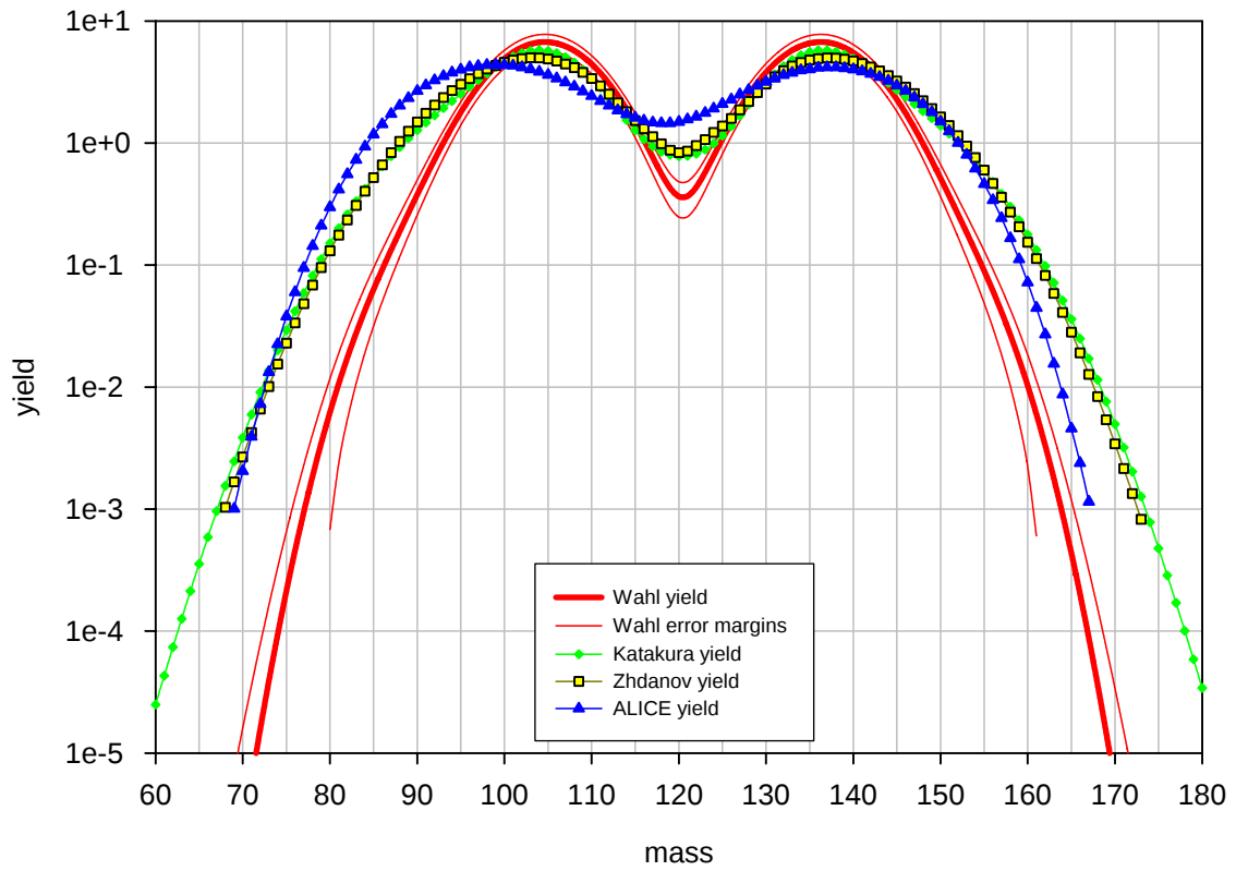
Benchmark B: ^{244}\text{Cm} at 13 MeV, post neutron emission mass distribution
